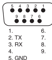
Figure 2–6 Interface RS-232C
